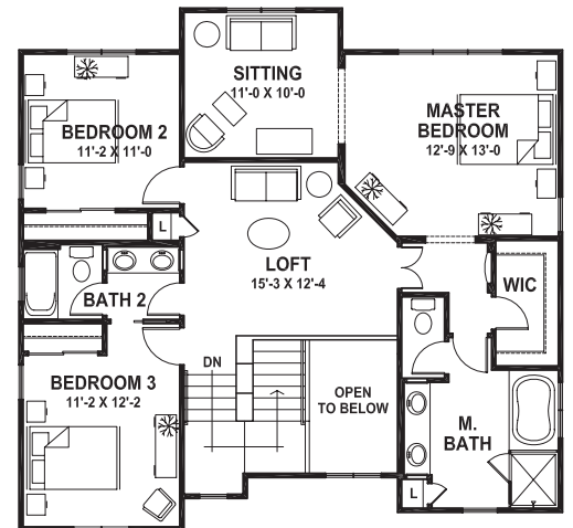
OPTIONAL MASTER SITTING ROOM
