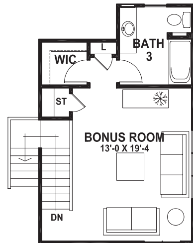
OPTIONAL SECOND FLOOR SUITE 4
